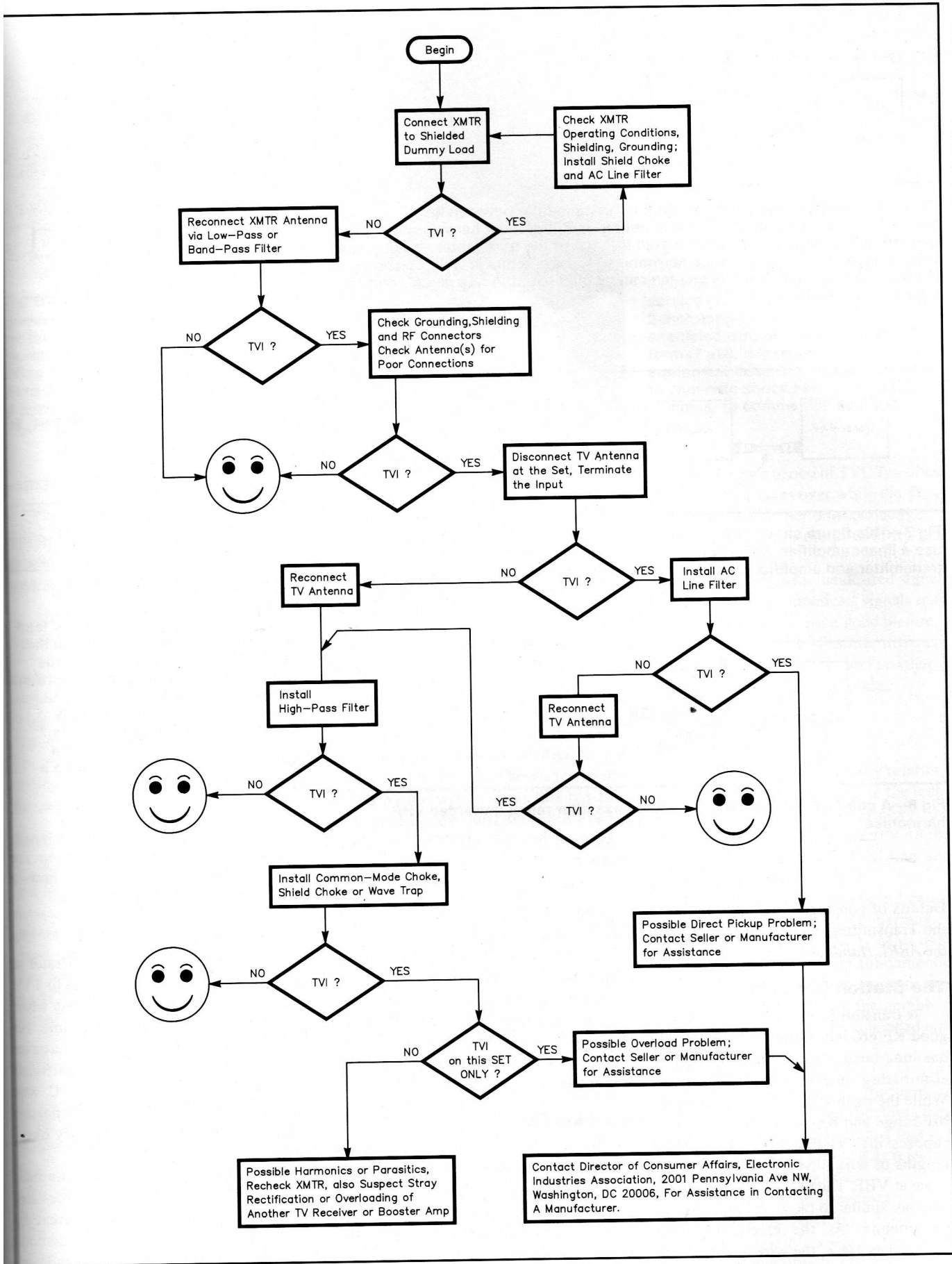
Fig 5—TVI troubleshooting flow chart.
